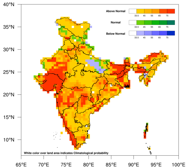
Fig.2a. Probability forecast of Maximum Temperature over India during November 2026.
