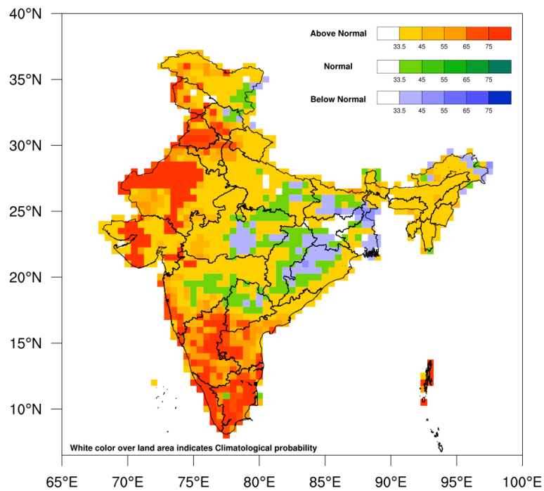
Fig.2b. Probability forecast of Minimum Temperature over India during November 2026.
