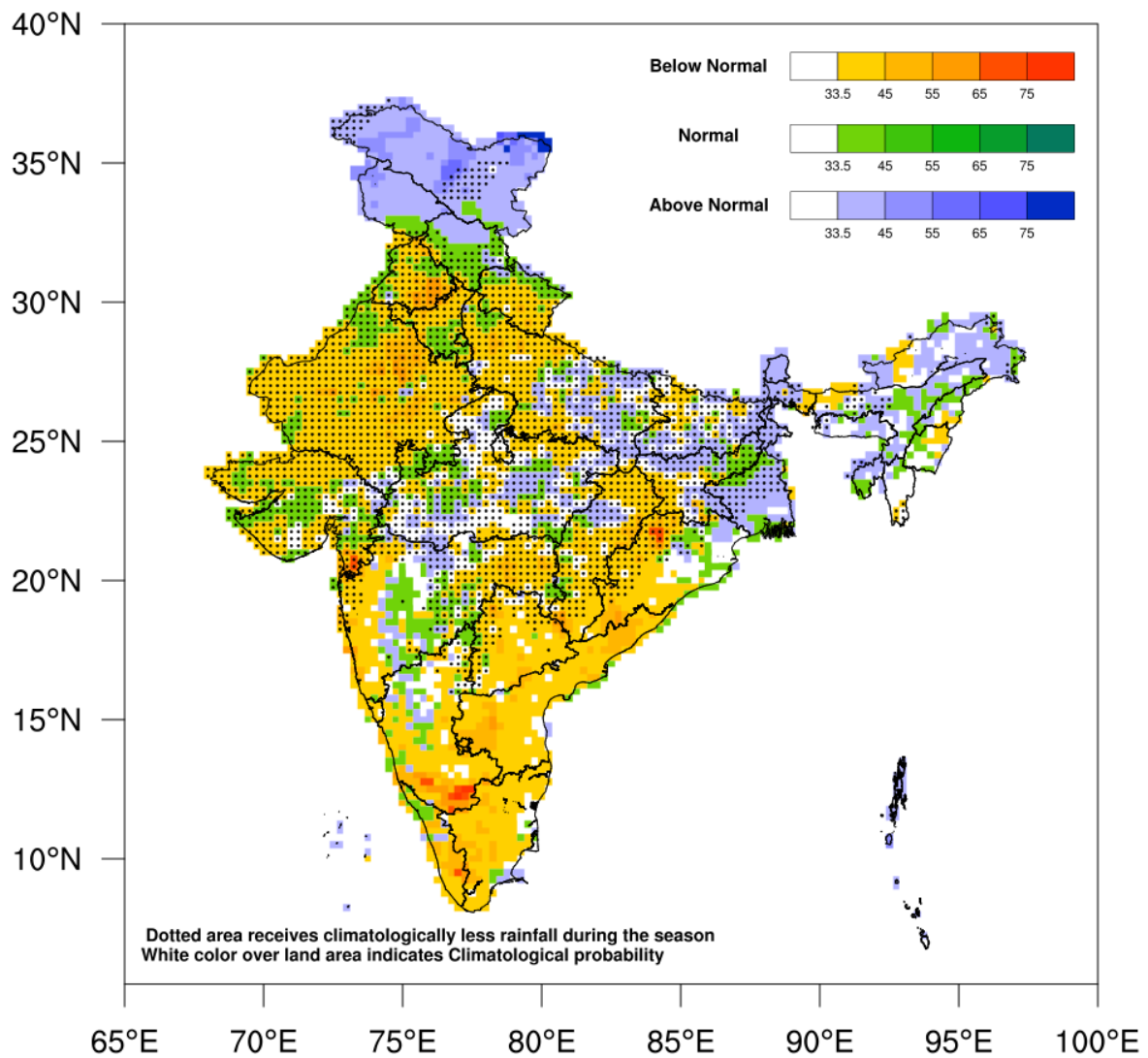
Fig.1. Probability forecast of rainfall in tercile categories* (below normal, normal, and above normal) over India during November, 2026. The figure illustrates the most likely categories as well as their probabilities. The dotted areas shown in the map climatologically receive very less rainfall during November and the white-shaded areas over the land represent no forecast signal by the model. (*Tercile categories have equal climatological probabilities of 33.33% each).
