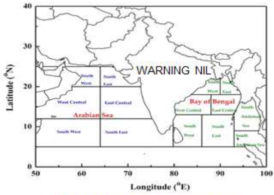
DAY-3: 28.01.2021/0600 UTC TO 29.01.2021/0600 UTC
