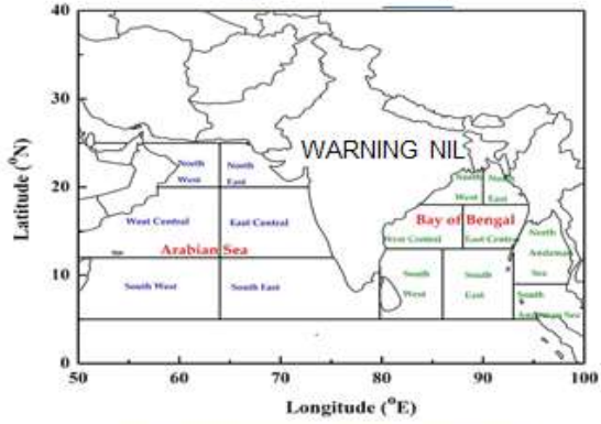
DAY-5: 30.01.2021/0600 UTC TO 31.01.2021/0600 UTC
