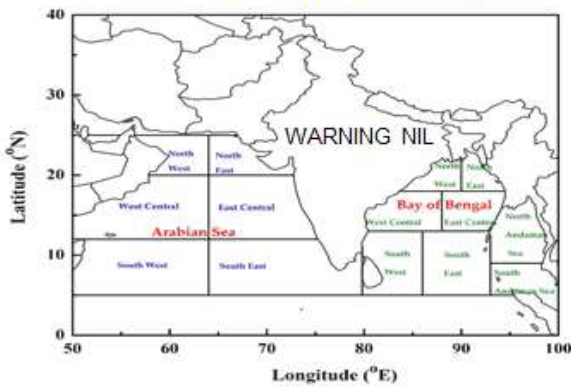
DAY-5: 30.01.2021/0600 UTC TO 31.01.2021/0600 UTC
