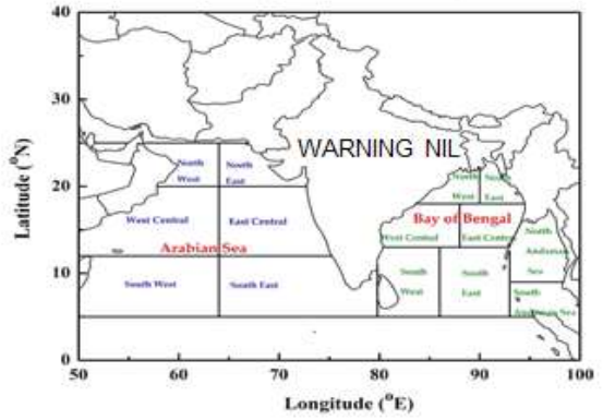
DAY-4: 29.01.2021/0600 UTC TO 30.01.2021/0600 UTC
