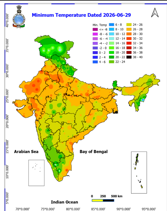
Fig. 3: Minimum Temperatures
