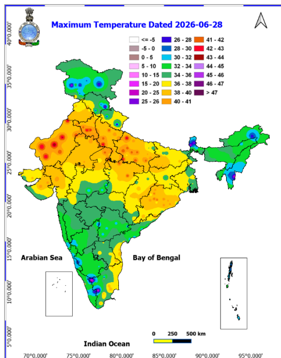
Fig. 1: Maximum Temperatures
