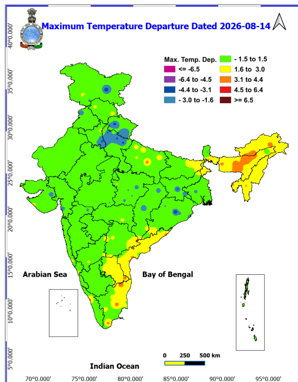
Fig. 2: Departure of Maximum Temp. Dated 2026-08-14
