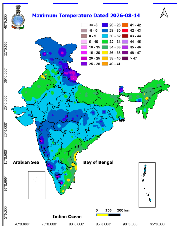
Fig. 1: Maximum Temperatures Dated 2026-08-14
