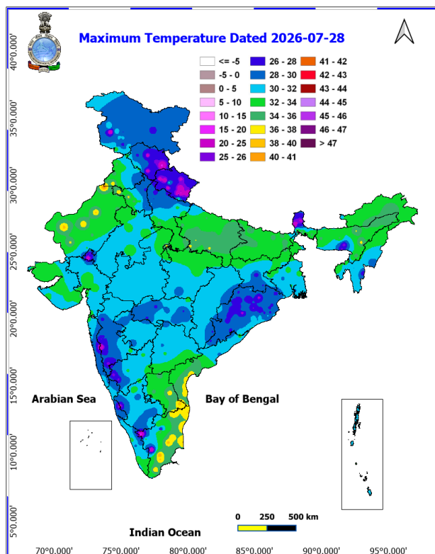
Fig. 1: Maximum Temperatures Dated 2026-07-28
