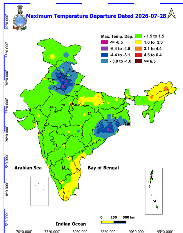
Fig. 2: Departure of Maximum Temp. Dated 2026-07-28
