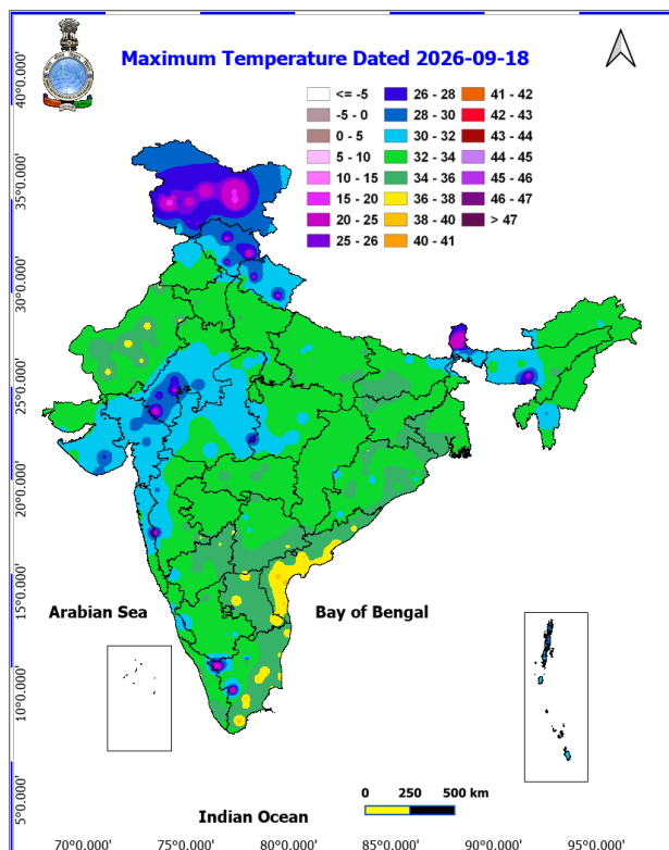
Fig. 1: Maximum Temperatures Dated 2026-09-18
