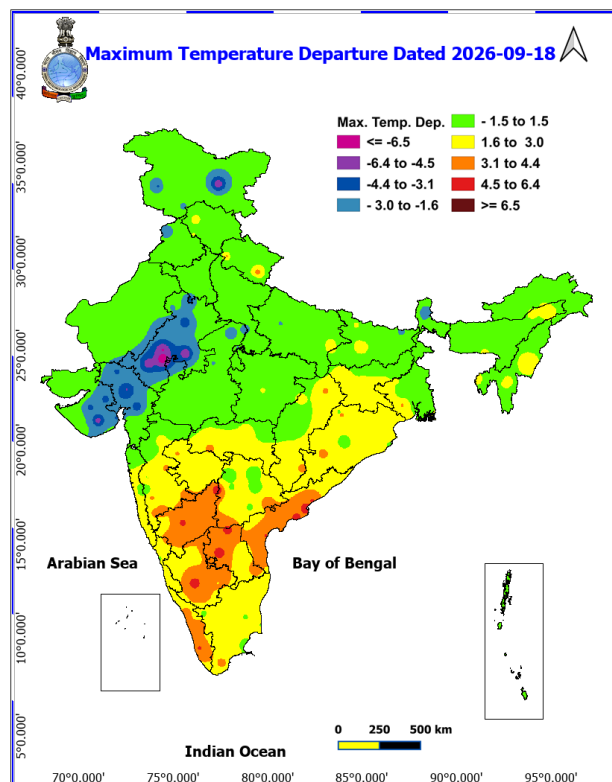
Fig. 2: Departure of Maximum Temp. Dated 2026-09-18
