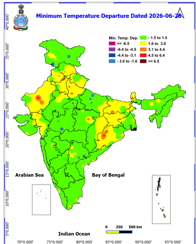
Fig. 4: Departure of Minimum Temp. Dated 2026-06-28
