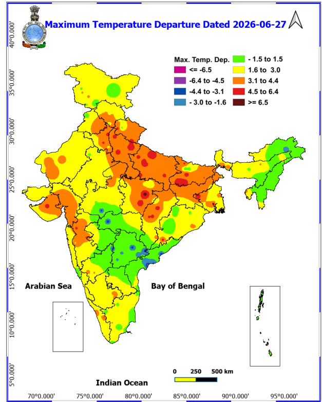
Fig. 2: Departure of Maximum Temp. Dated 2026-06-27
