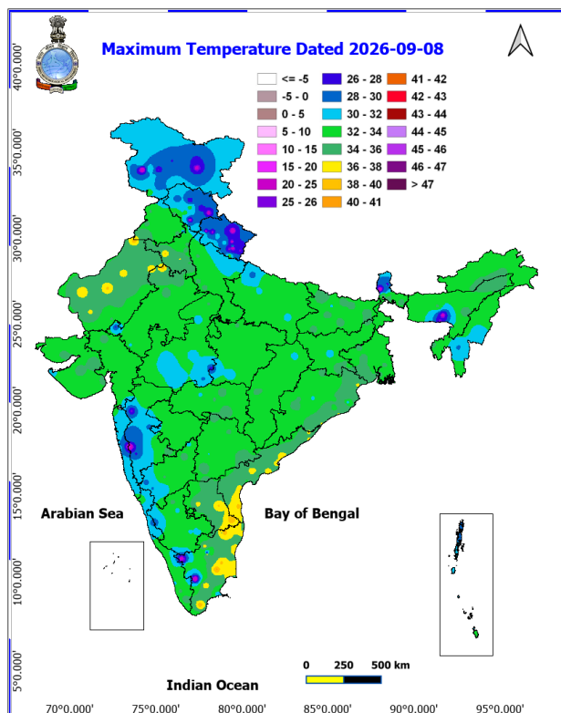
Fig. 1: Maximum Temperatures Dated 2026-09-08
