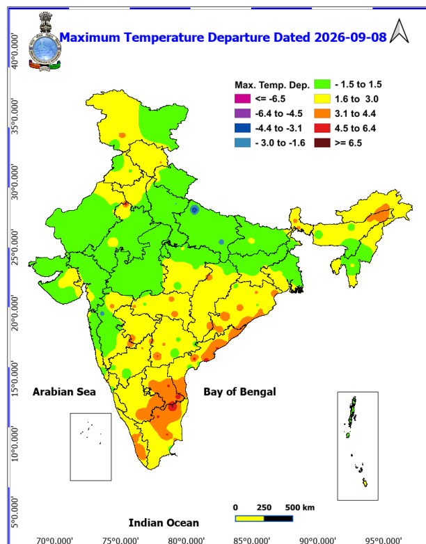
Fig. 2: Departure of Maximum Temp. Dated 2026-09-08
