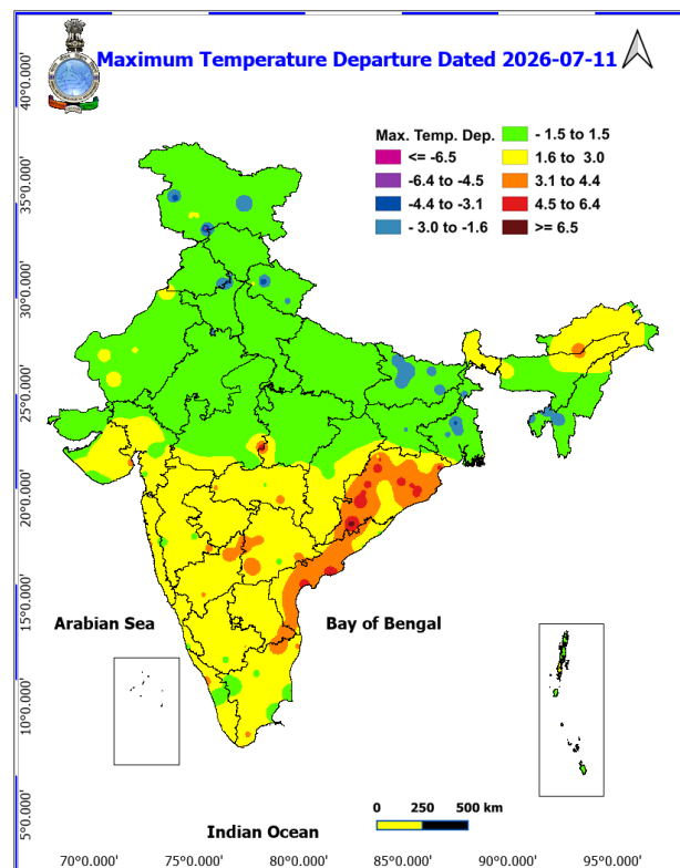
Fig. 2: Departure of Maximum Temp. Dated 2026-07-11
