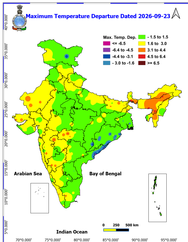
Fig. 2: Departure of Maximum Temp. Dated 2026-09-23
