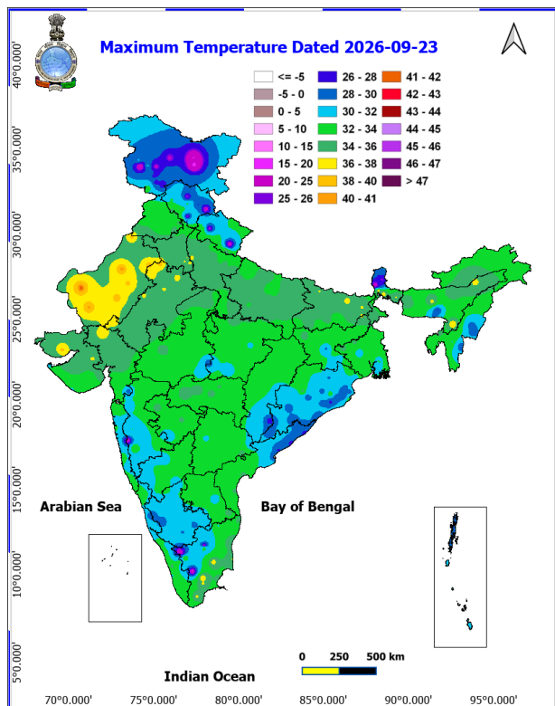
Fig. 1: Maximum Temperatures Dated 2026-09-23
