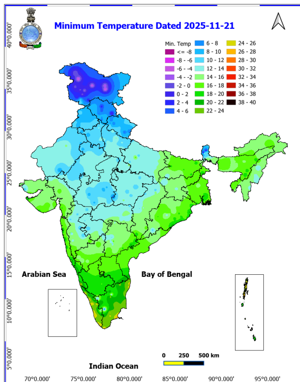
Fig. 3: Minimum Temperatures Dated 2025-11-21
