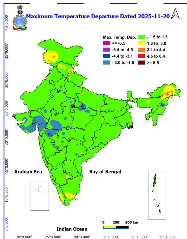
Fig. 2: Departure of Maximum Temp. Dated 2025-11-20
