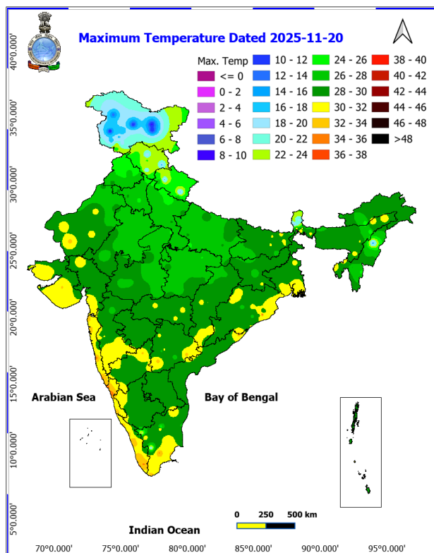
Fig. 1: Maximum Temperatures Dated 2025-11-20
