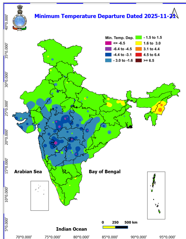
Fig. 4: Departure of Minimum Temp. Dated 2025-11-21
