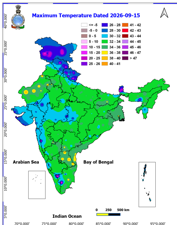
Fig. 1: Maximum Temperatures Dated 2026-09-15
