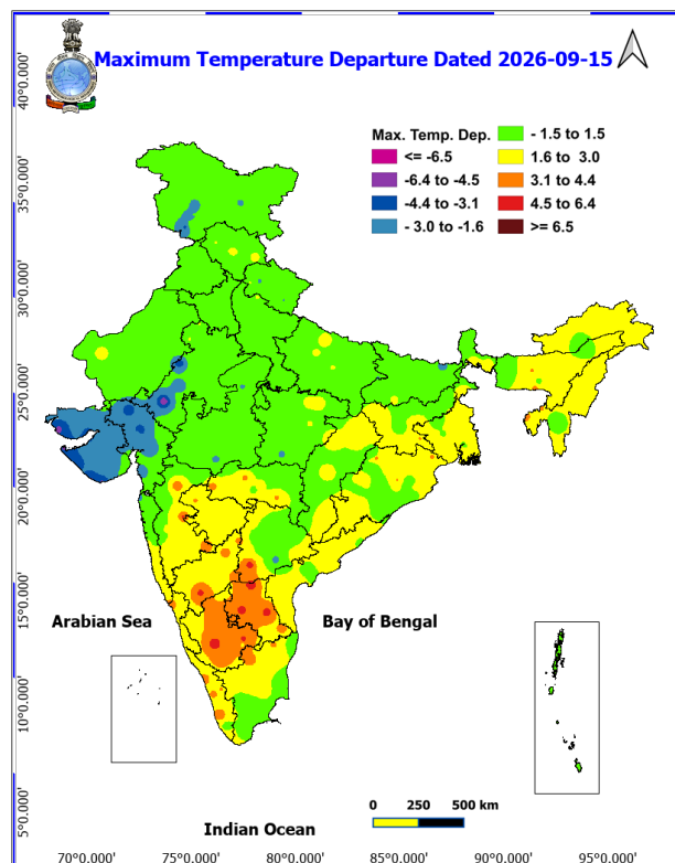
Fig. 2: Departure of Maximum Temp. Dated 2026-09-15
