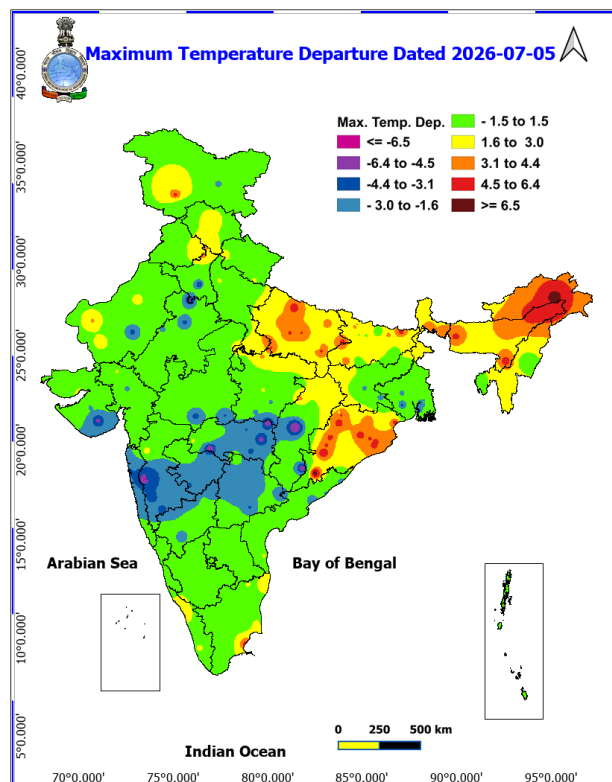
Fig. 2: Departure of Maximum Temp. Dated 2026-07-05
