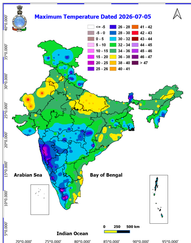
Fig. 1: Maximum Temperatures Dated 2026-07-05
