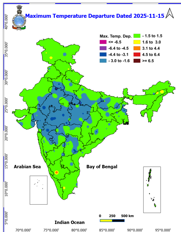
Fig. 2: Departure of Maximum Temp. Dated 2025-11-15
