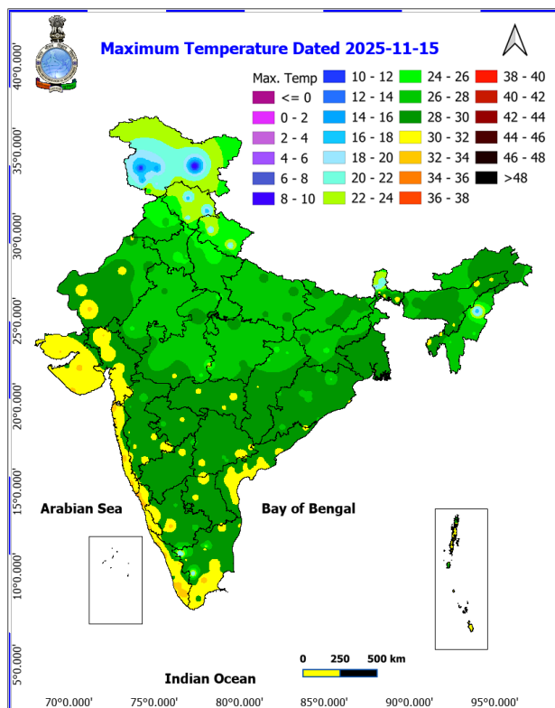
Fig. 1: Maximum Temperatures Dated 2025-11-15
