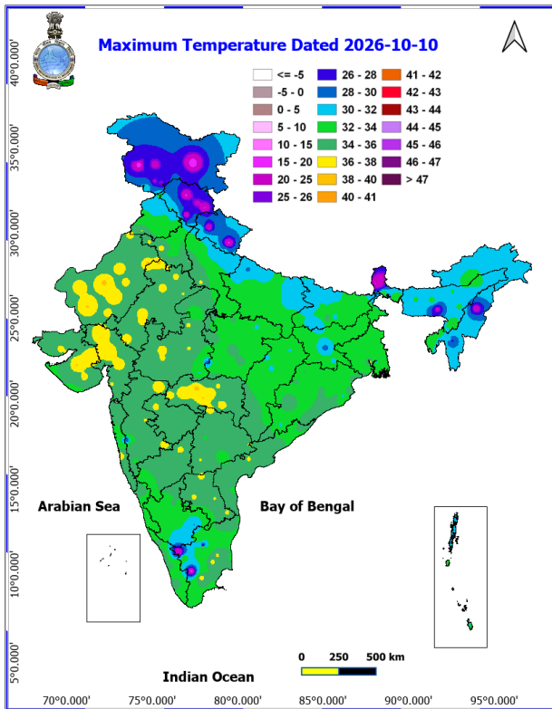
Fig. 1: Maximum Temperatures Dated 2026-10-10
