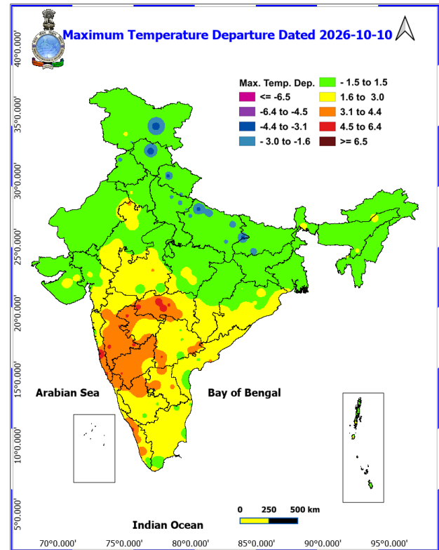
Fig. 2: Departure of Maximum Temp. Dated 2026-10-10
