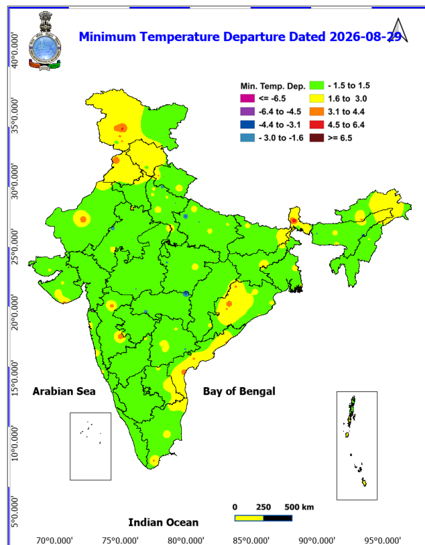
Fig. 4: Departure of Minimum Temp. Dated 2026-08-29
