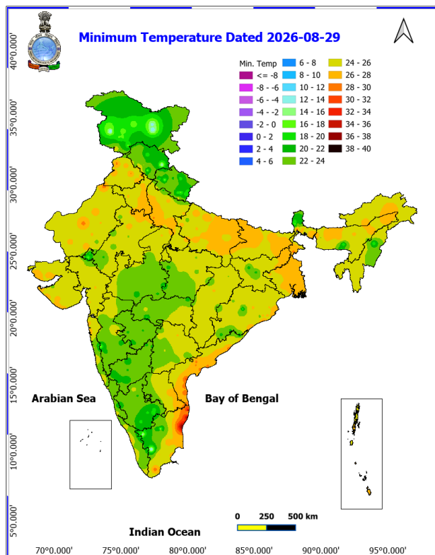
Fig. 3: Minimum Temperatures Dated 2026-08-29
