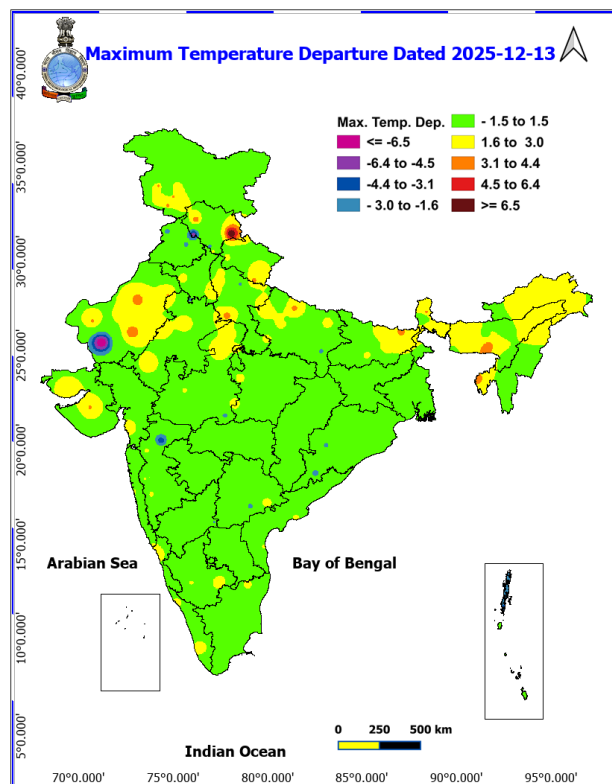
Fig. 2: Departure of Maximum Temp. Dated 2025-12-13
