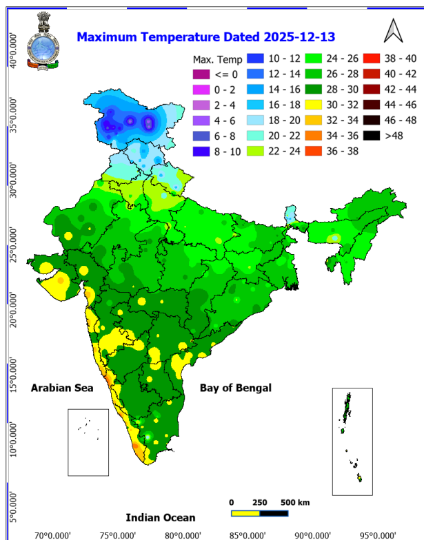
Fig. 1: Maximum Temperatures Dated 2025-12-13
