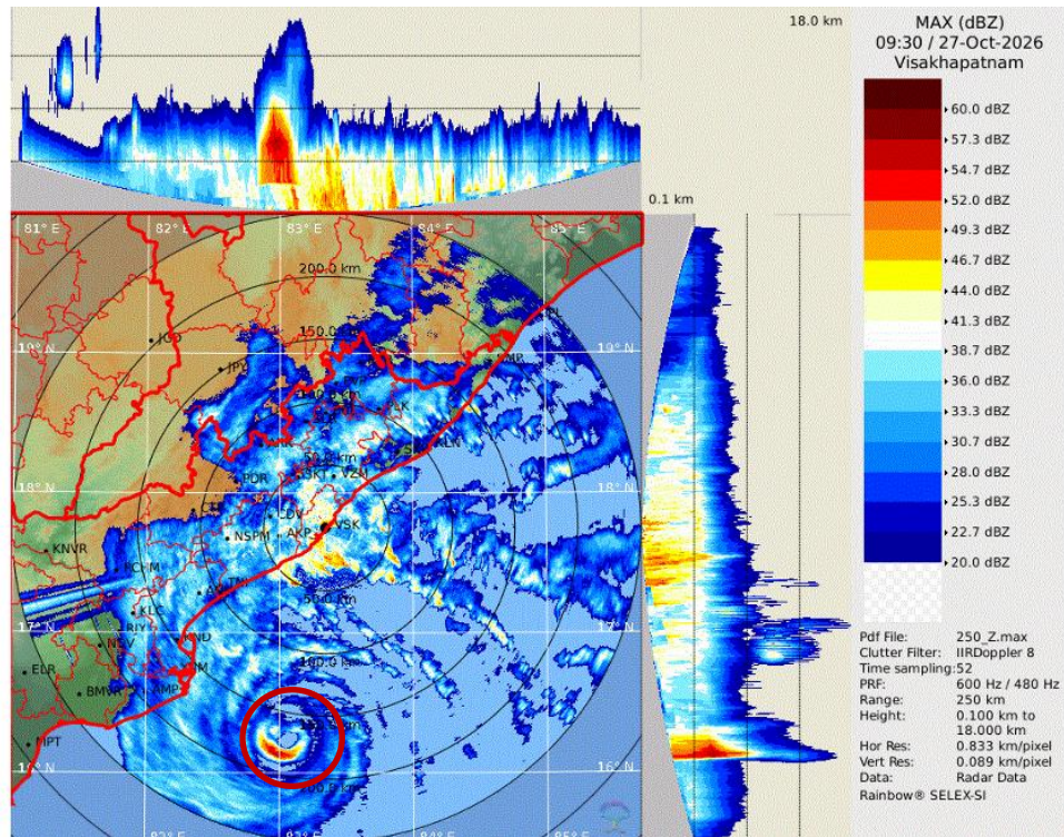
Radar Image of Vishakhapatnam at 1500 hrs IST of 27 th Oct 2026
