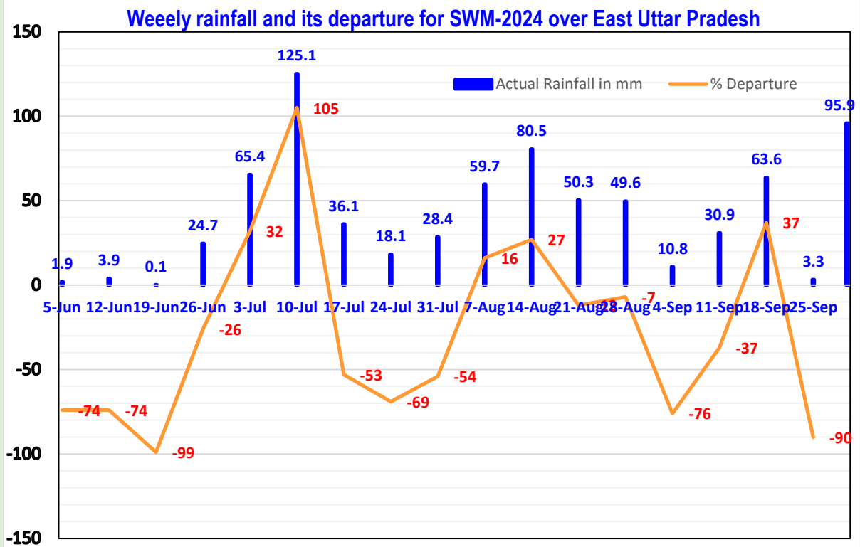
Figure 8 Weekly Rainfall & its Departure for SWM 2024 over East Uttar Pradesh
