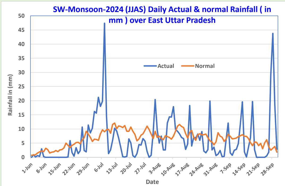
Figure 17: Daily Actual & normal rainfall time series of East Uttar Pradesh
