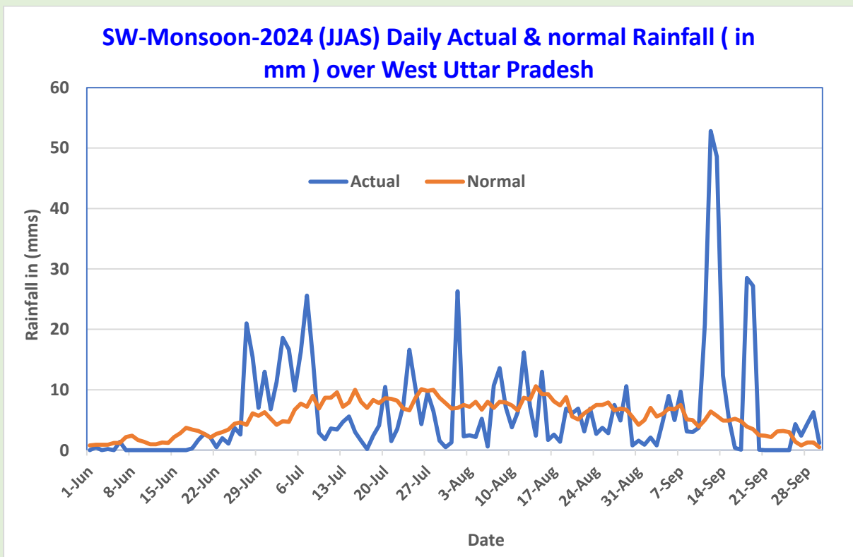
Figure 18: Daily Actual & normal rainfall time series of West Uttar Pradesh
