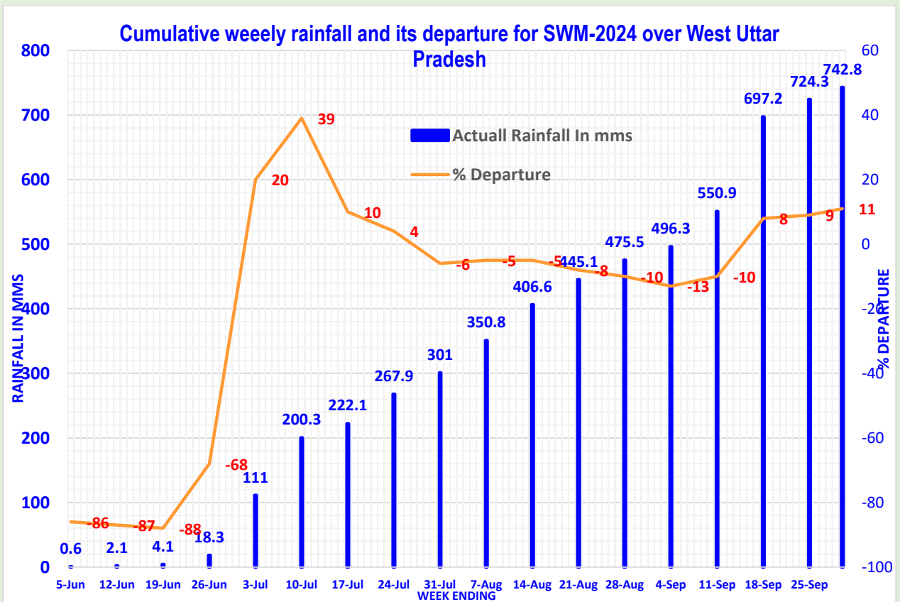
Figure 12: Cumulative Weekly Rainfall & its Departure for SWM 2024 over West Uttar Pradesh
