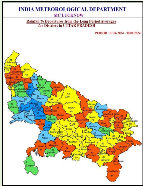
Figure 3: District wise Rainfall map for the month of June-2024
