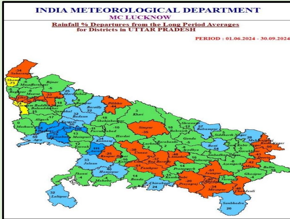
Figure 7: District wise Rainfall map for Monsoon Season (JJAS)-2024
