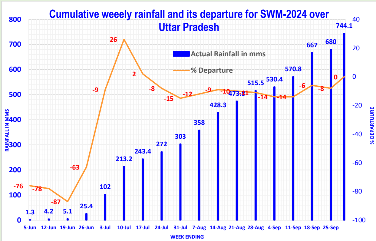
Figure 13: Cumulative Weekly Rainfall & its Departure for SWM 2024 over Uttar Pradesh
