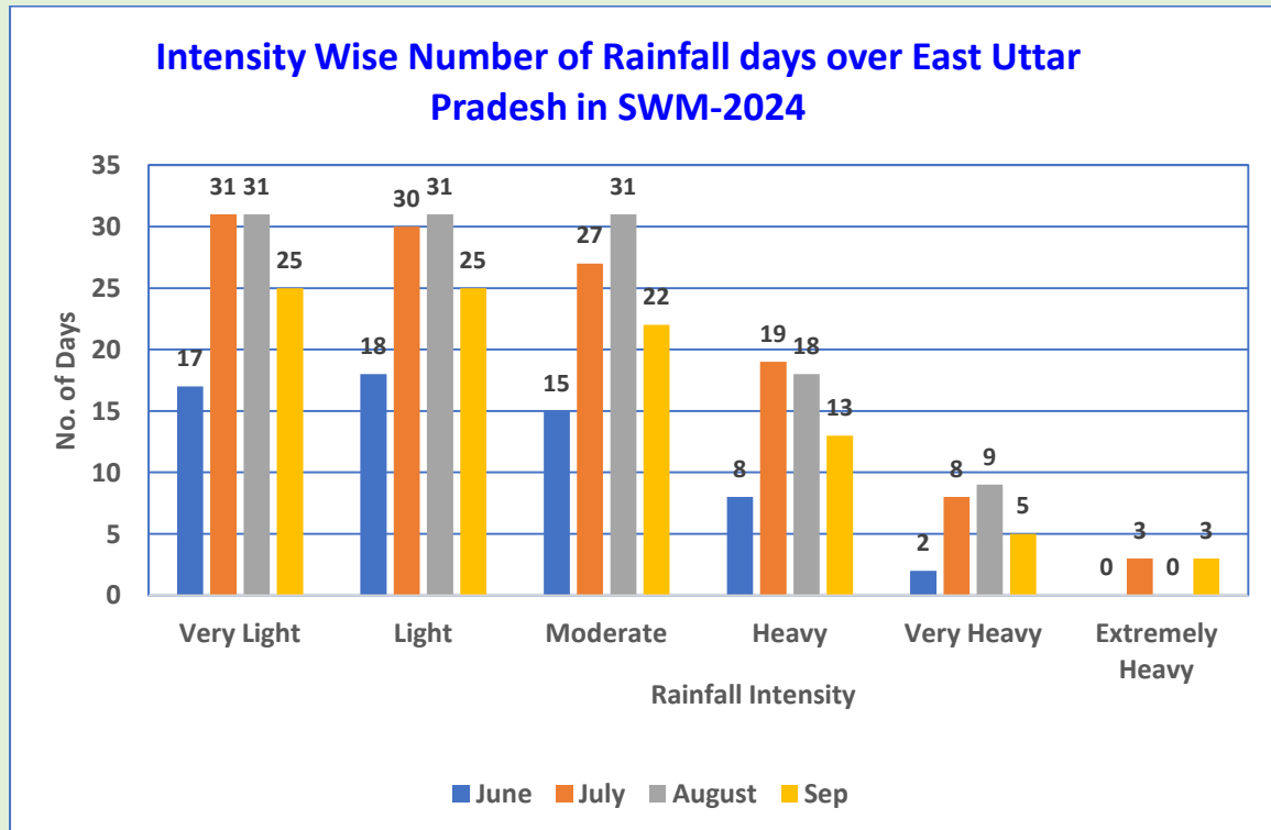
Figure 14: Month-wise and intensity-wise number of rainfall days over East Uttar Pradesh
