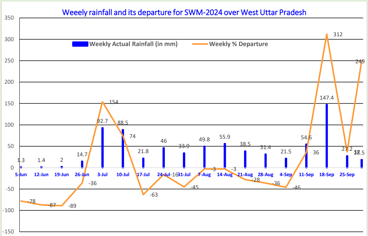
Figure 9: Weekly Rainfall & its Departure for SWM 2024 over West Uttar Pradesh
