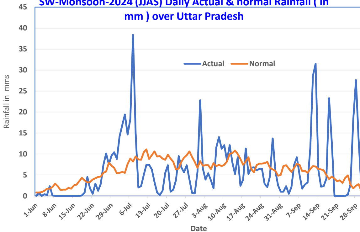
Figure 16: Daily Actual & normal rainfall time series of Uttar Pradesh
