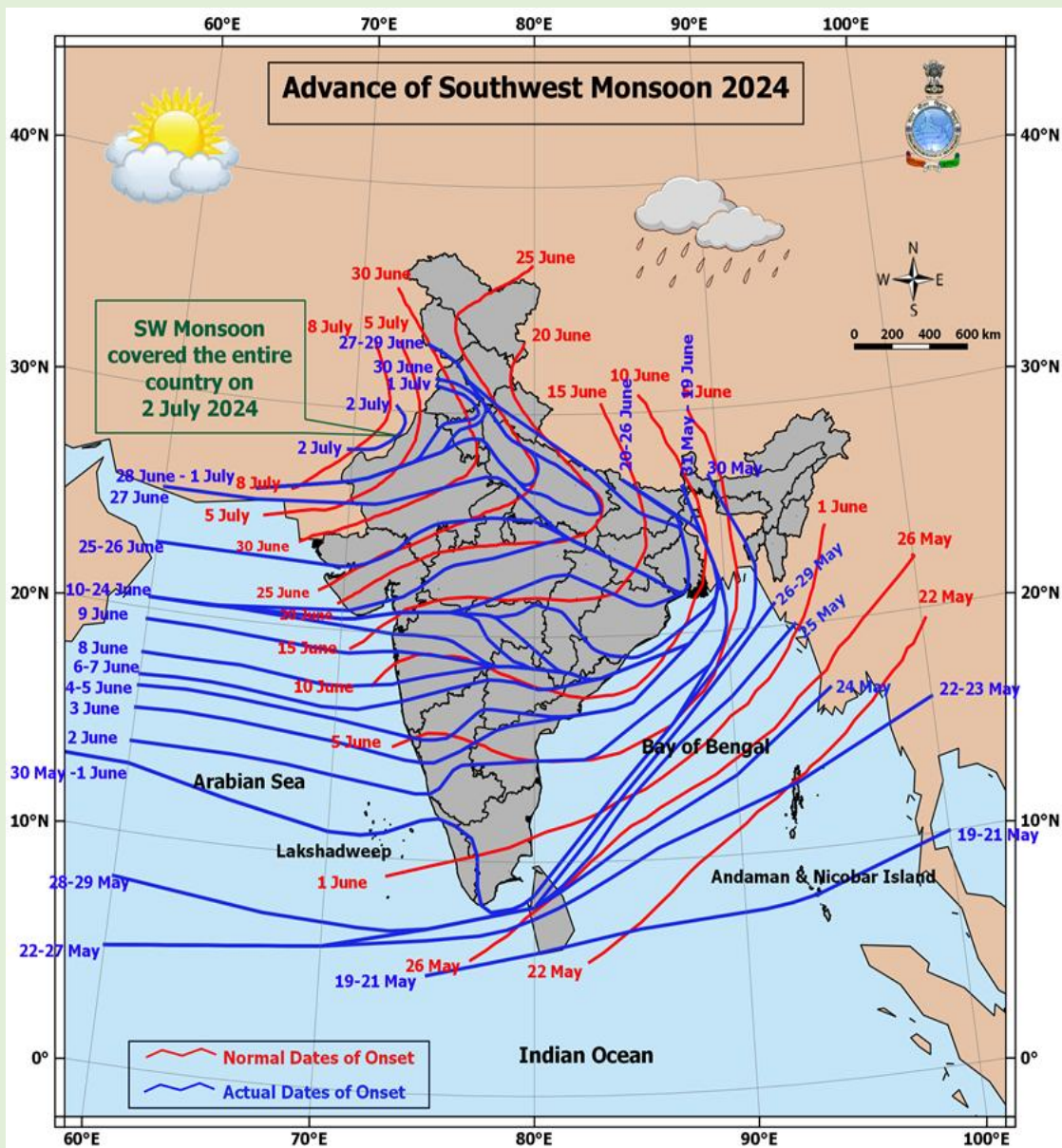
Figure 1: Advance of Southwest Monsoon-2024
