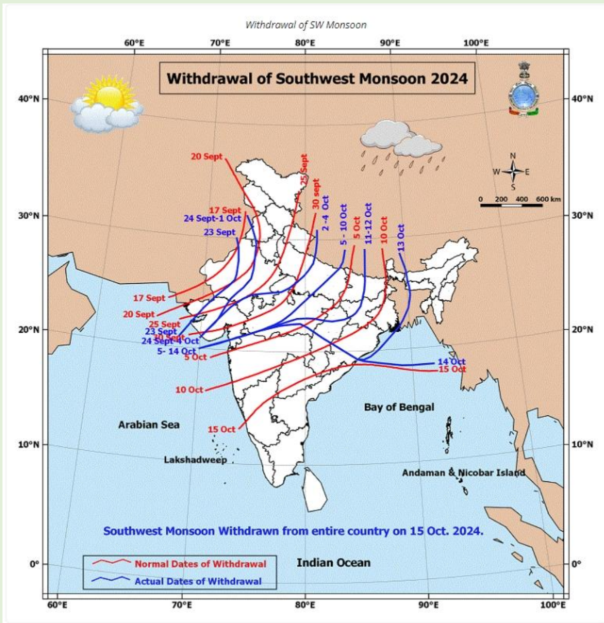
Figure 2: Withdrawal of Southwest Monsoon 2024
