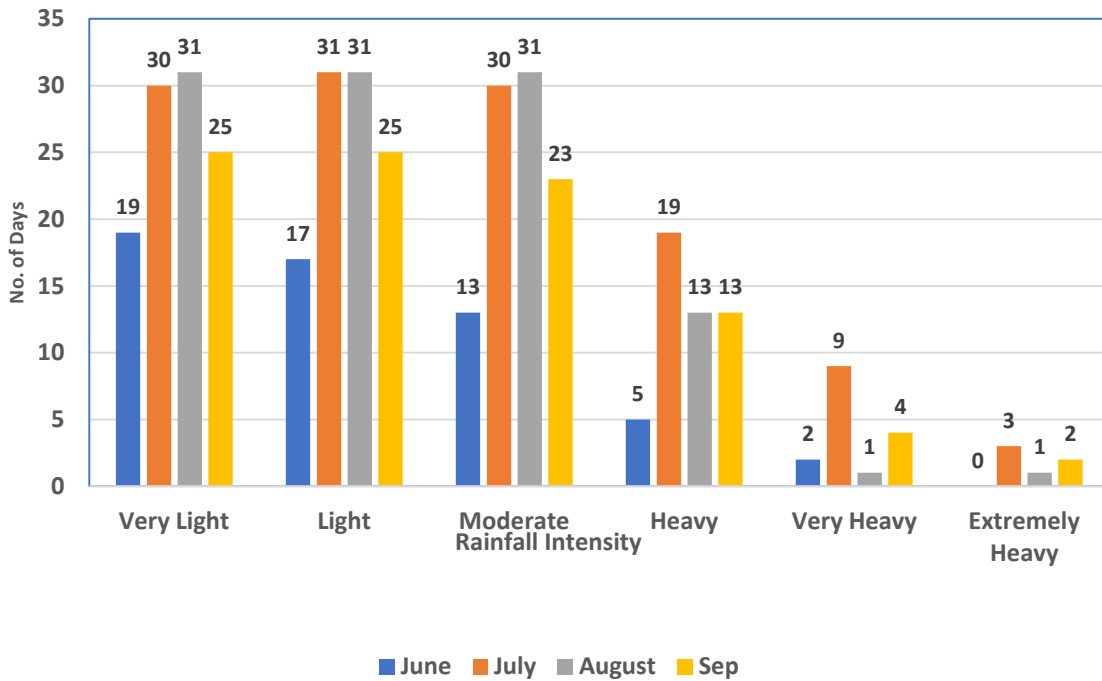
Figure 15: Month-wise and intensity-wise number of rainfall days over West Uttar Pradesh
